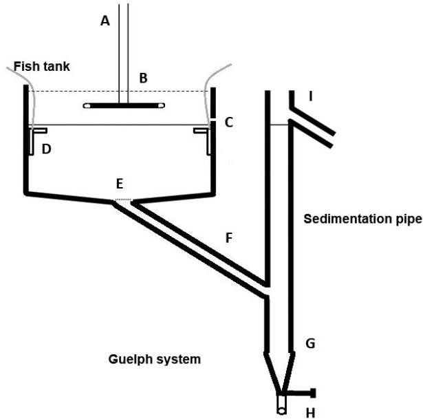
Fig. 3. Scheme of the Guelph system consisting of a connection of a fish tank and sedimentation tube. A = inflow water from biofilter tank (fitted with a T-shaped showerhead; clockwise); B = net covering of fish tank; C = overflow of any excess water from fish tank (directly into reservoir tank underneath); D = air pipes fitted with fish tank wall (in clockwise direction) and supplied with air tubes from air pump; E = sieve at the central outlet drain of fish tank (slightly sloped bottom); F = transport tube for water and solids from fish tank to sedimentation pipe; G = conical silo at the bottom of sedimentation tube for trapping sedimented solids; H = tap for draining trapped solids or feces; I = outflow of clear water (supernatant) post sedimentation of solids (into bottom reservoir tank).
